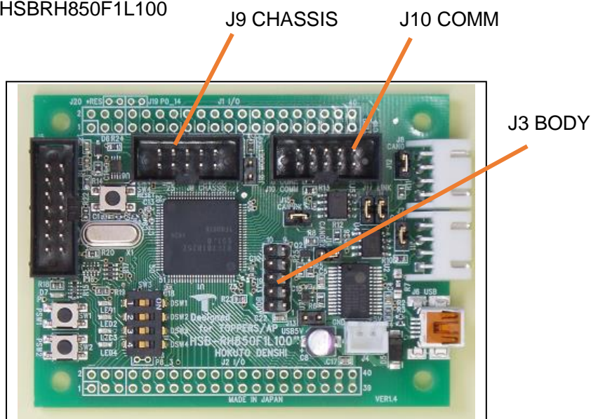
HSBRH850F1L100
