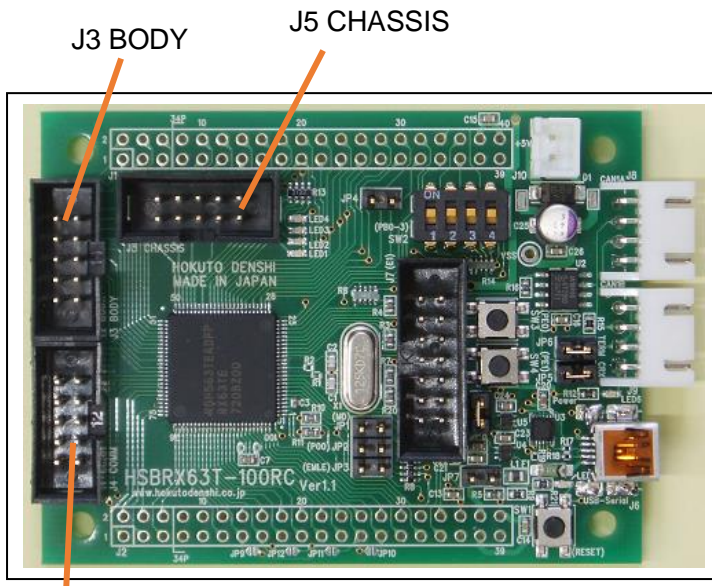
HSBRX63T100-RC
